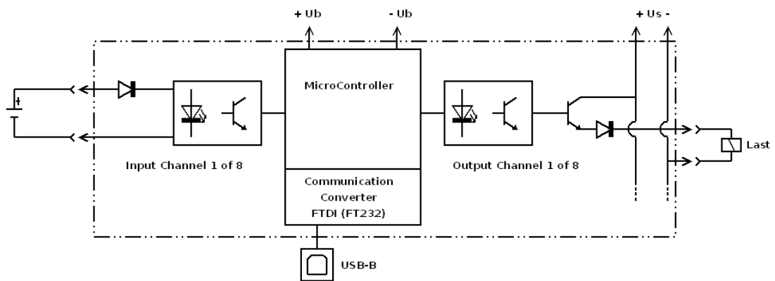
Schematic Diagram
