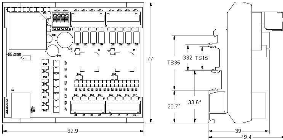
Dimensions (mm)
